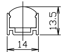
FN2-BRACKET1 取付図
