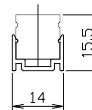
FN2-BRACKET1 取付図
