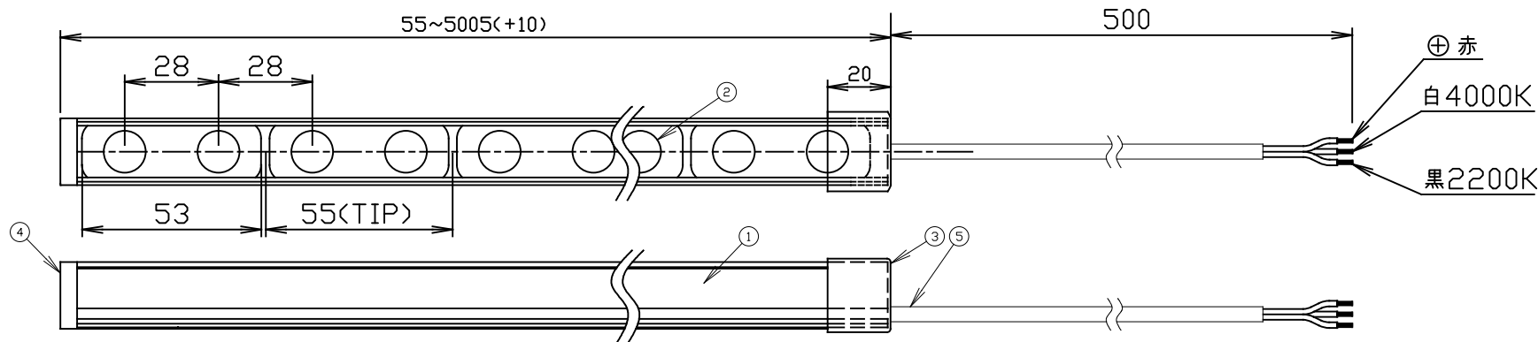
FNL3D-EXL FNL3D-EXL-FLEX 取付図
