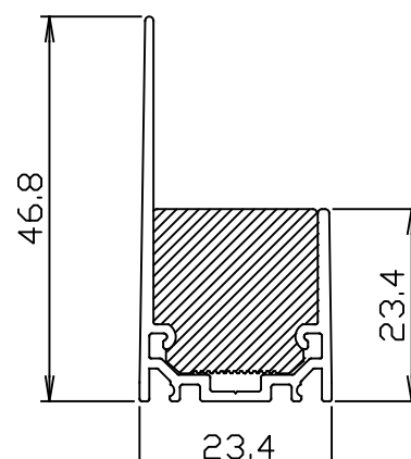
FNL3D-EXL-FLEX-AG 取付図
