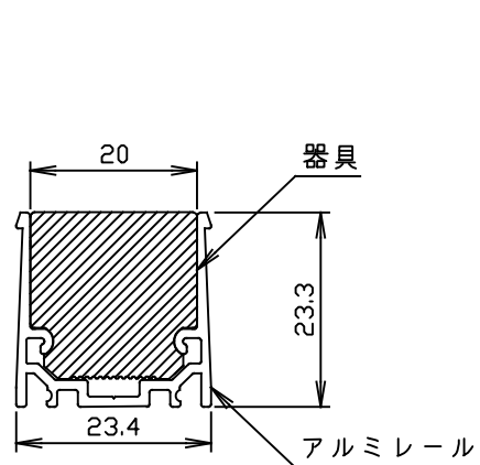
FNL3D-EXL FNL3D-EXL-FLEX 取付図
