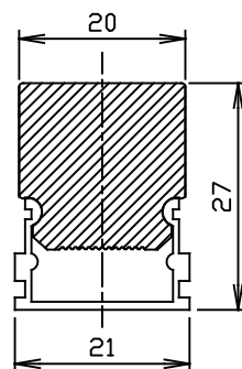
FNL3D-BRACKET1 取付図
