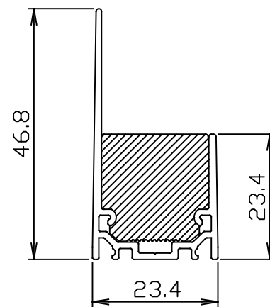
FNL3D-EXL-FLEX-AG 取付図
