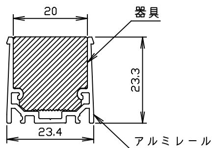
FNL3D-EXL FNL3D-EXL-FLEX 取付図
