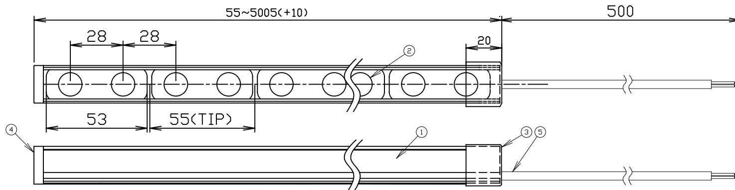
FNL3D-EXL FNL3D-EXL-FLEX 取付図
