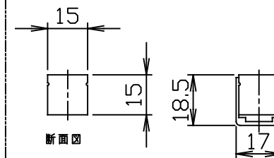
FN3D-EXL FN3D-EXL-FLEX FN3D-BRACKET1 取付図
